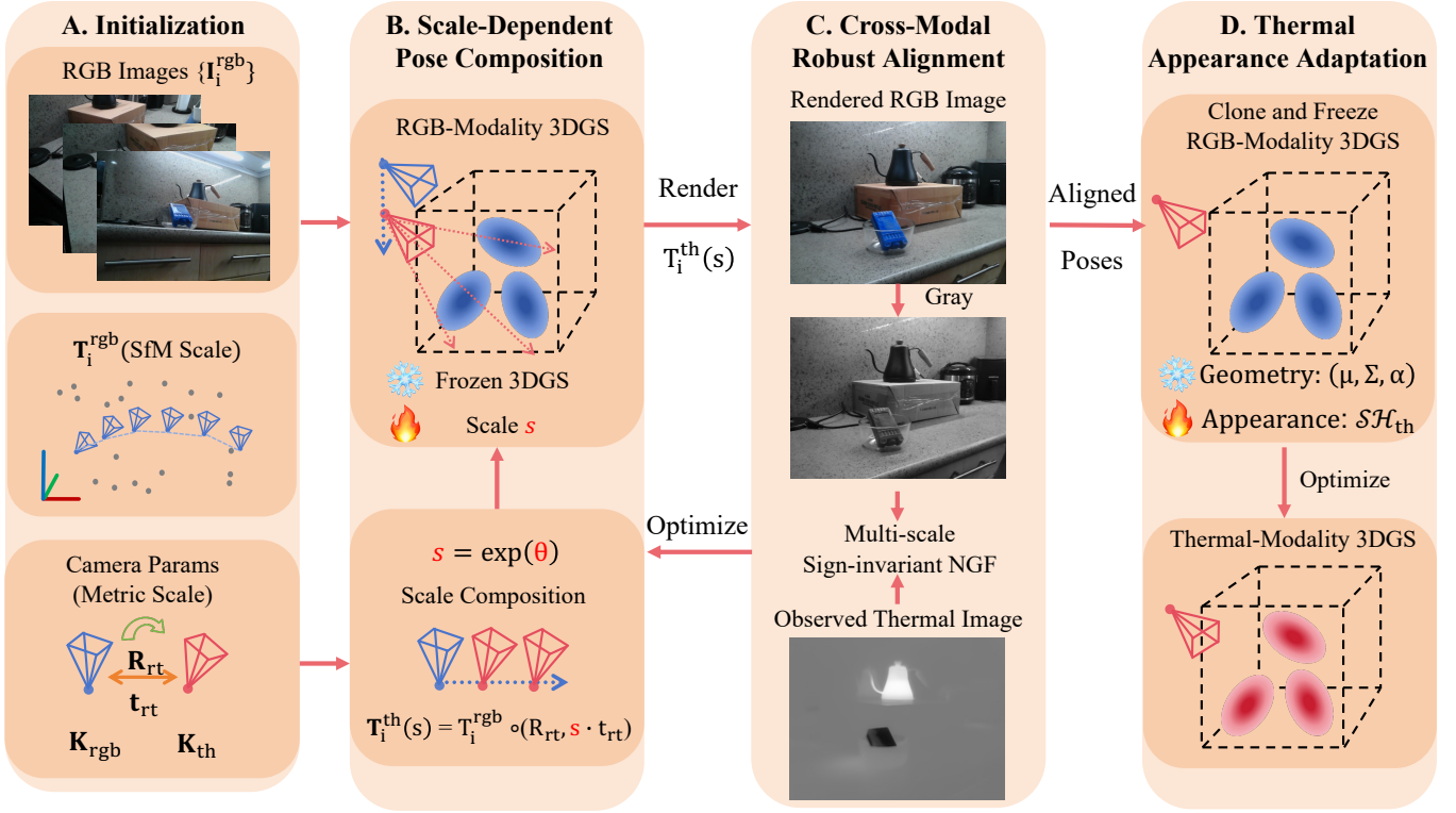
Fig. 2. Overview of our proposed method. We first train an RGB-3DGS model (Sec. III-B). To align the thermal sensors with the scale-ambiguous RGB reconstruction, we optimize a global scale factor s by minimizing a sign-invariant gradient loss between thermal images and grayscale RGB renderings (Sec. III-C). Finally, we adapt the model to the thermal modality by learning thermal spherical harmonics on the frozen geometry (Sec. III-D).
