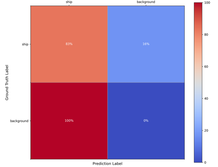
Fig. 5: Confusion matrix for our model.
