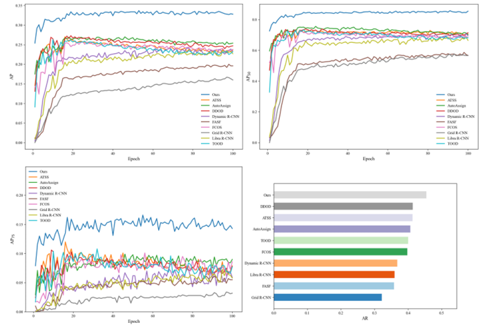
Fig. 2: Performance comparison of object detection algorithms across epochs.
