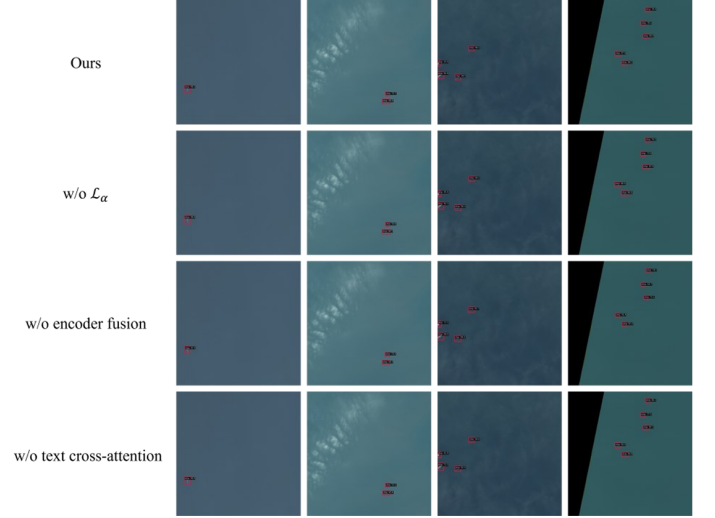
Fig. 4: Comparisons of the detection results by different methods.
