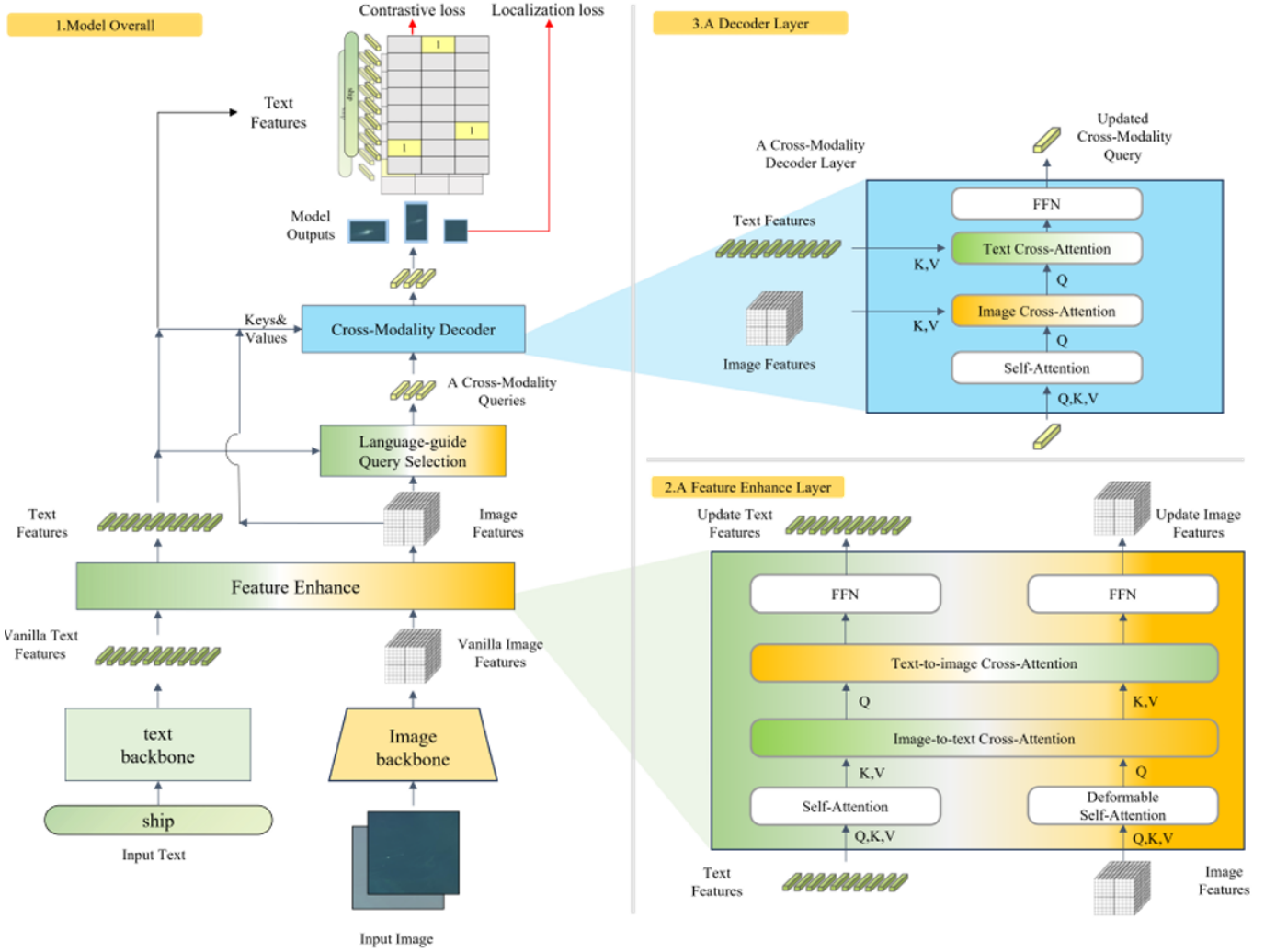
Fig. 1: The framework of our model.
