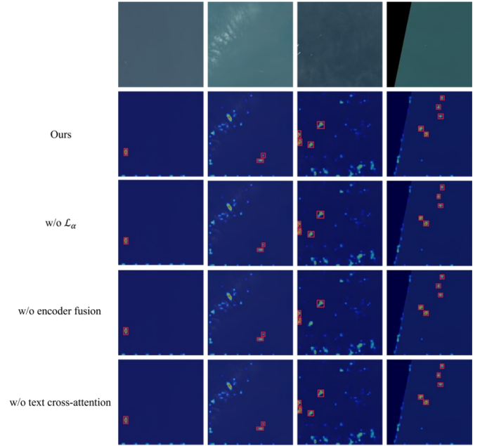
Fig. 3: Heatmaps from ablation experiments of our model.
