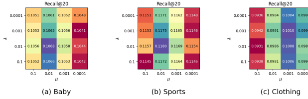
Fig. 4: Performance Landscape over (\lambda, \mu) .
