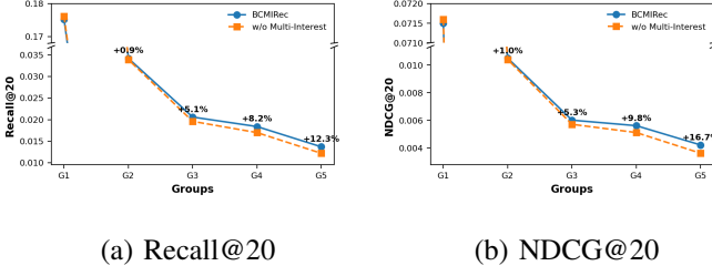
Fig. 2: Long-tail performance across item popularity groups on Sports.
