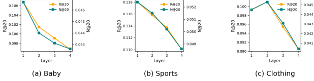
Fig. 3: Sensitivity to Propagation Depth L .
