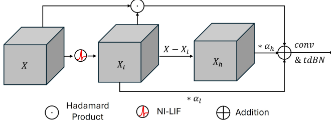
Fig. 5. The illustration of the frequency decomposition module.
